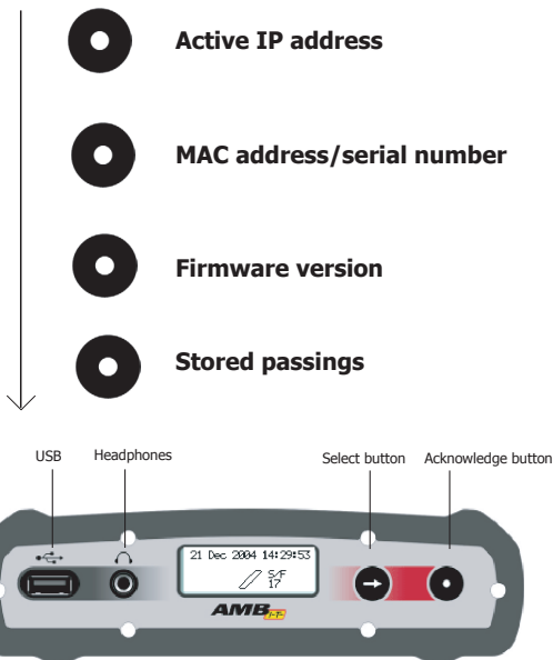
Figure 1.4: Decoder with status display
