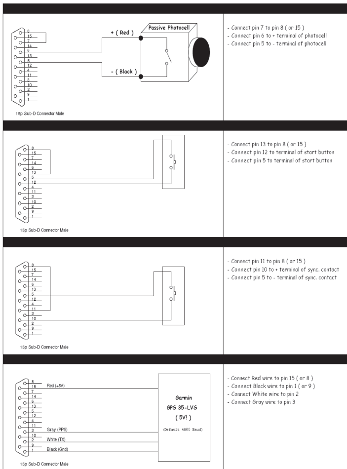
Figure 1.7: Connecting photocells, connection setup
