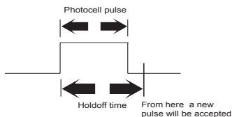
Figure 1.6 Holdoff time
