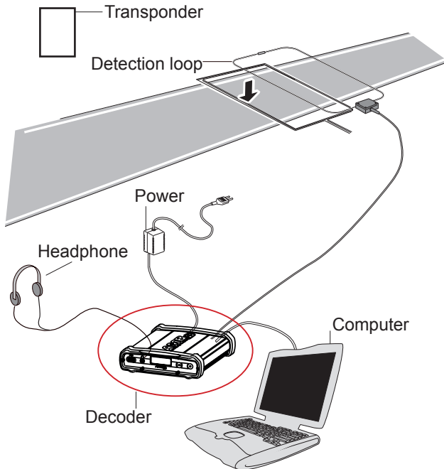
Figure 1.1 System overview
